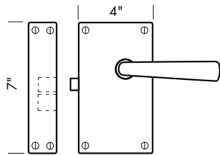
CS-RL300-PA -Complete rim lock with spindle. -Passage set. -Shown with L-106 lever.
