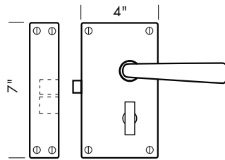
CS-RL300-PR -Complete rim lock with spindle. -Privacy set. -Shown with L-106 lever.
