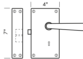
CS-RL300-BK -Complete rim lock with bit key and spindle. -Shown with L-106 lever.
