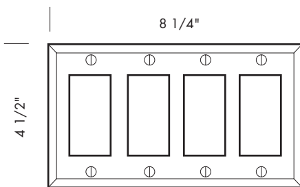
EC-304 8 1/4" x 4 1/2" 4-gang decora cover.
