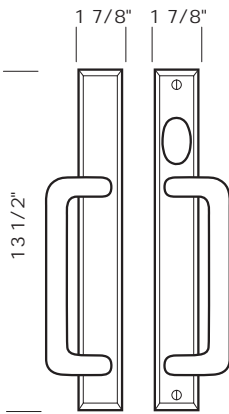
CMPUS-816SLPF -Complete set with turn piece. -Patio function.
