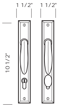
CMP-811SL -Complete set with keyed profile cylinder, SVB turn piece and spindle. -Single cylinder. -Shown with L-107 lever.
