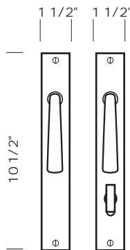
CMP-980SL-PF -Complete set with 1/2 profile cylinder, SVB turn piece, and spindle. -Patio function. -Shown with L-106 lever.
