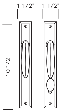
CMP-811SLPF -Complete set with 1/2 profile cylinder, SVB turn piece and spindle. -Patio function. -Shown with L-107 lever.
