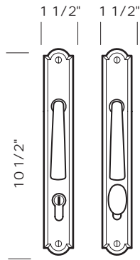
CMPA811SL -Complete set with keyed profile cylinder, SVB turn piece, and spindle. -Single cylinder. -Shown with L-106 lever.
