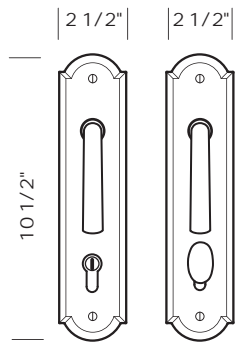
CMPA812SL -Complete set with keyed profile cylinder, SVB turn piece and spindle. -Single cylinder. -Shown with L-112 lever.
