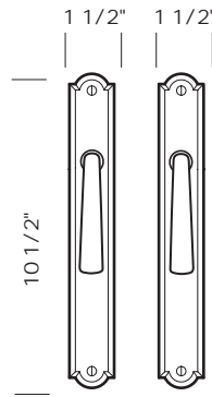
CMPA811SL-FD -Trim set only. -Full dummy. -Shown with L-106 lever.
