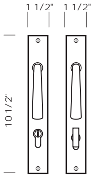
CMP-980SL -Complete set with keyed profile cylinder, SVB turn piece, and spindle. -Single cylinder. -Shown with L-106 lever.
