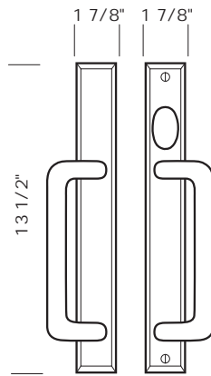
CMPUS-816SLPF -Complete set with turn piece. -Patio function.
