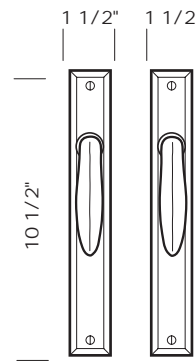
CMP-811SLFD -Trim set only. -Full dummy. -Shown with L-107 lever.
