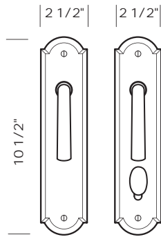
CMPA812SL-PF -Complete set with 1/2 profile cylinder, SVB turn piece and spindle. -Patio function. -Shown with L-112 lever.
