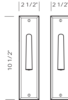
CMP-812SLFD -Trim set only. -Full dummy. -Shown with L-133 lever.
