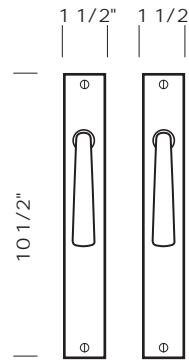
CMP-980SL-FD -Trim set only. -Full dummy. -Shown with L-106 lever.
