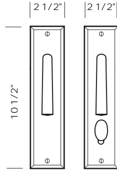
CMP-812SLPF -Complete set with 1/2 profile cylinder, SVB turn piece and spindle. -Patio function. -Shown with L-133 lever.
