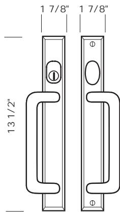
CMPUS-816SL -Complete set with keyed US cylinder, and turn piece. -Single cylinder.
